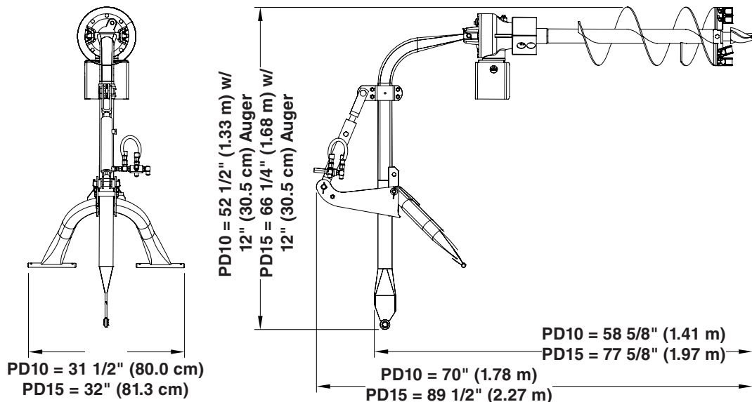
PD10 & PD15 Overall Dimensional Drawing
