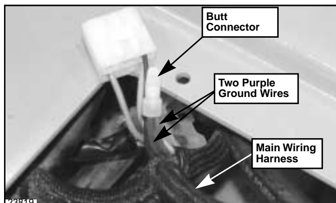
Installing Butt Connector Figure 7
