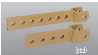
Some tractor and tire combinations do not allow enough room for the mower hook-up. Longer lower hitch clevises are available to easily correct this situation.
