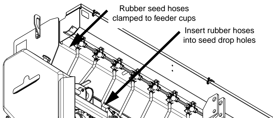
Small Seeds Tube Assembly Figure 1-4
