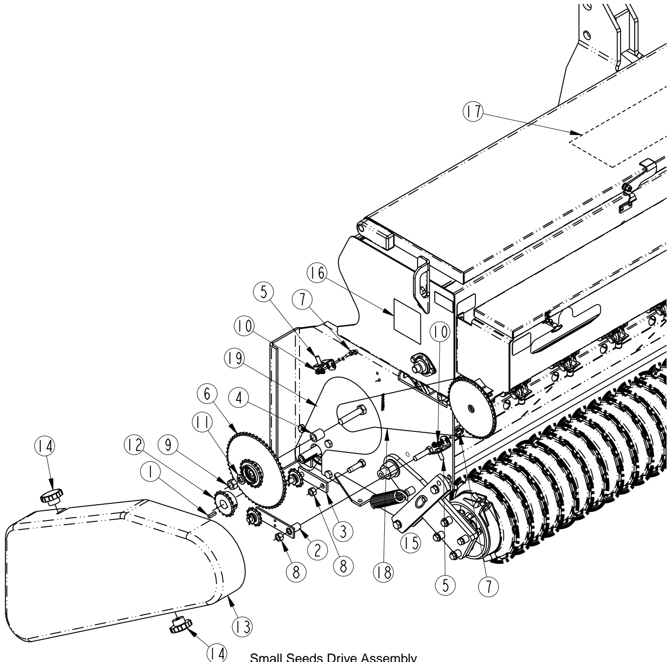
Small Seeds Drive Assembly Figure 1-8
